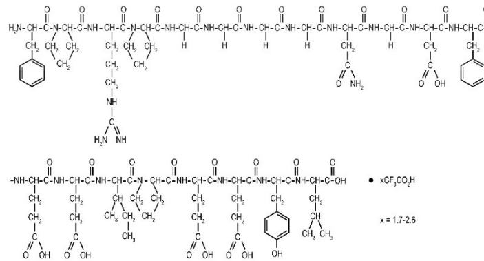
Figure 1. Structure formula for bivalirudin trifluoroacetate
