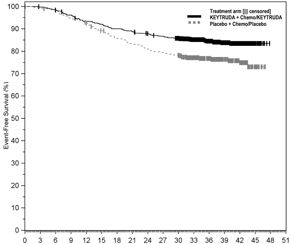
Figure 24: Kaplan-Meier Curve for Event-Free Survival in KEYNOTE-522
