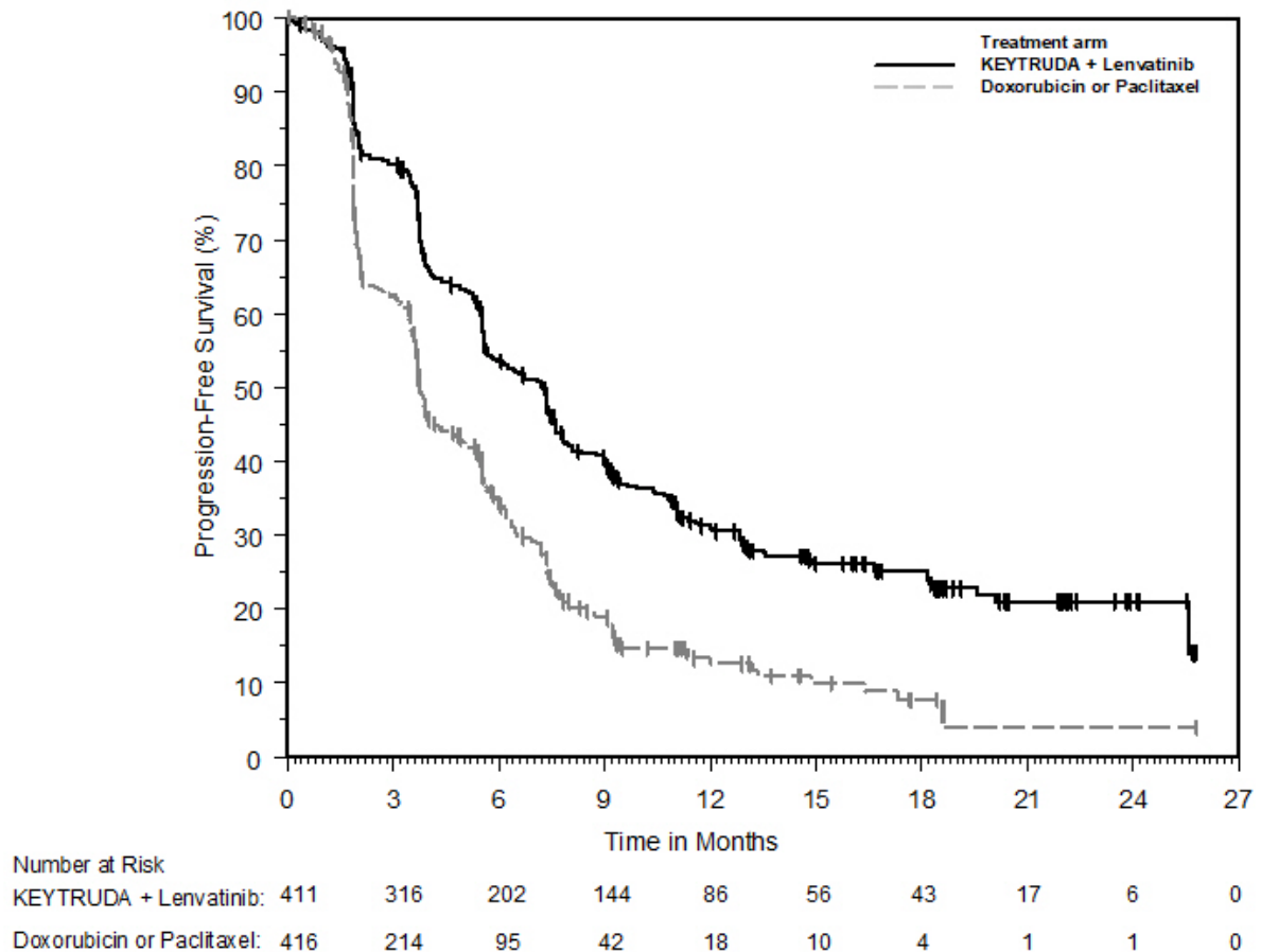
Figure 23: Kaplan-Meier Curve for Progression-Free Survival in KEYNOTE-775
