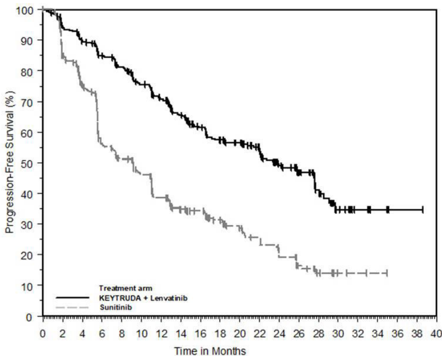
Figure 19: Kaplan-Meier Curve for PFS in KEYNOTE-581
