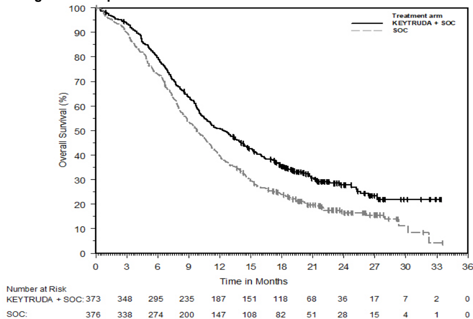
Figure 14: Kaplan-Meier Curve for Overall Survival in KEYNOTE-590
