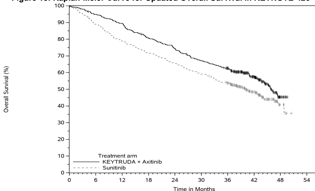
Figure 18: Kaplan-Meier Curve for Updated Overall Survival in KEYNOTE-426
