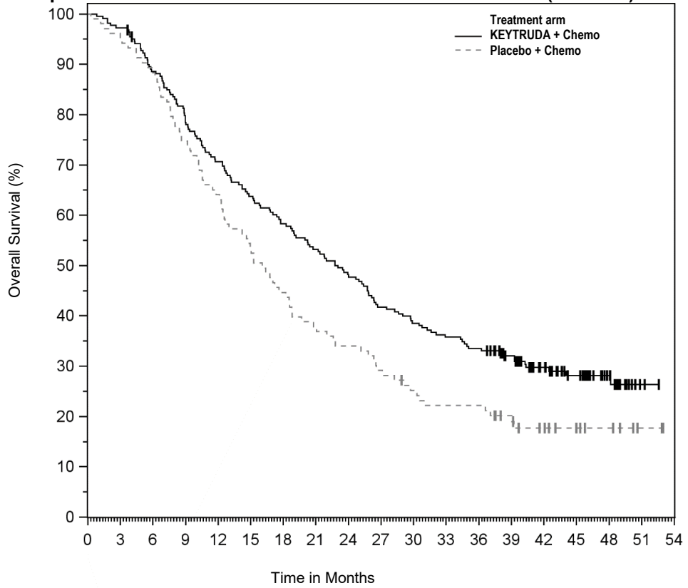
Figure 25: Kaplan-Meier Curve for Overall Survival in KEYNOTE-355 (CPS \geq 10 )
