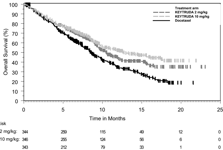
Figure 8: Kaplan-Meier Curve for Overall Survival in all Randomized Patients in KEYNOTE 010 (TPS ≥1%)
