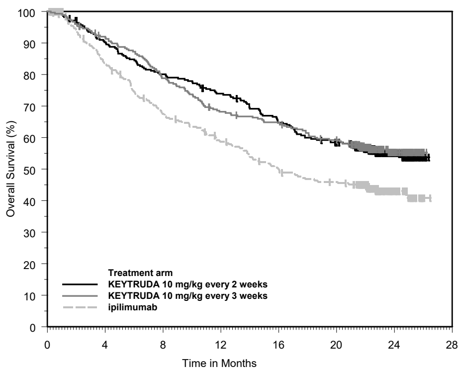
Figure 1: Kaplan-Meier Curve for Overall Survival in KEYNOTE 006*
