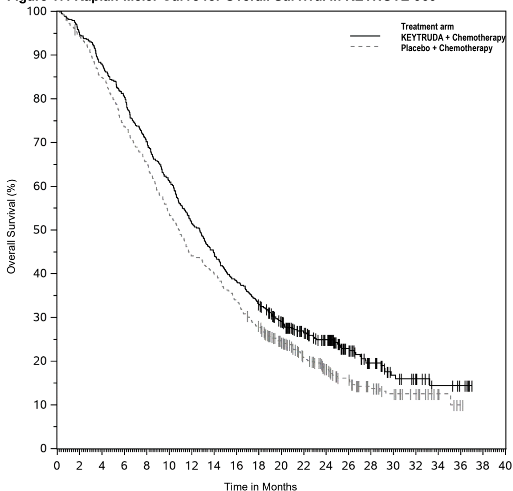
Figure 17: Kaplan-Meier Curve for Overall Survival in KEYNOTE-966
