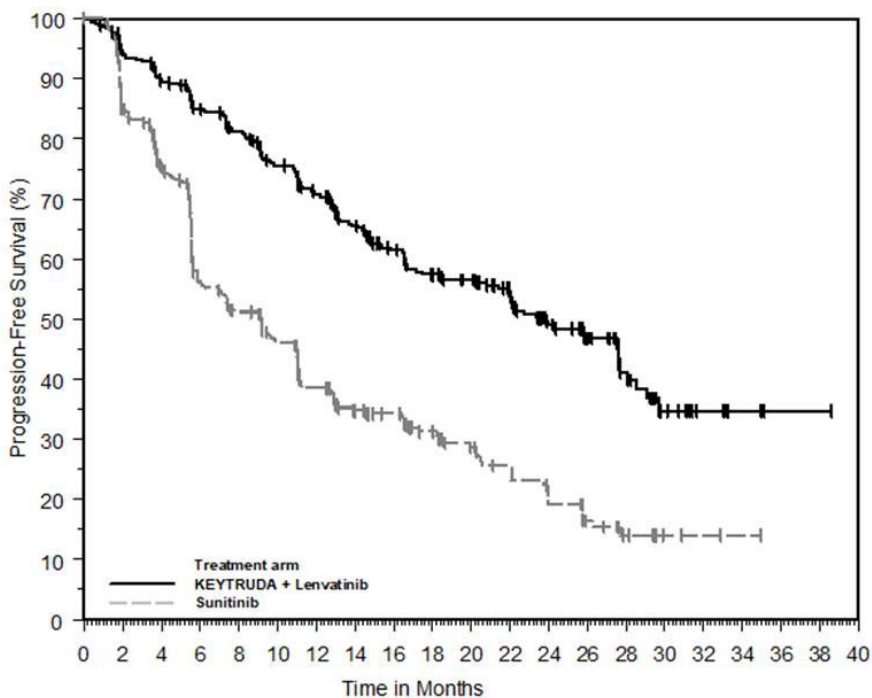
Figure 20: Kaplan-Meier Curve for PFS in KEYNOTE-581
