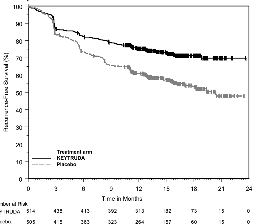
Figure 4: Kaplan-Meier Curve for Recurrence-Free Survival in KEYNOTE-054
