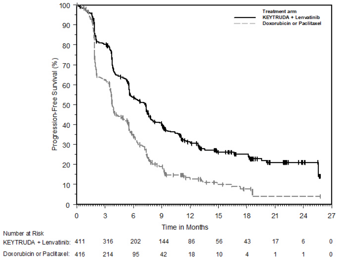
Figure 24: Kaplan-Meier Curve for Progression-Free Survival in KEYNOTE-775
