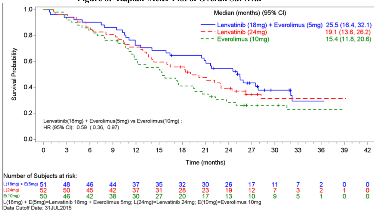
Figure 8: Kaplan-Meier Plot of Overall Survival
