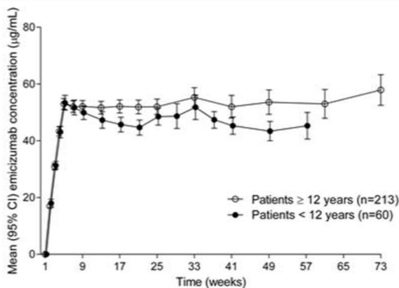
Figure 1: Mean ( \pm 95% CI) plasma emicizumab concentration versus time profiles for patients \geq 12 years (studies HAVEN 1 and HAVEN 3) compared with patients < 12 years (study HAVEN 2)
