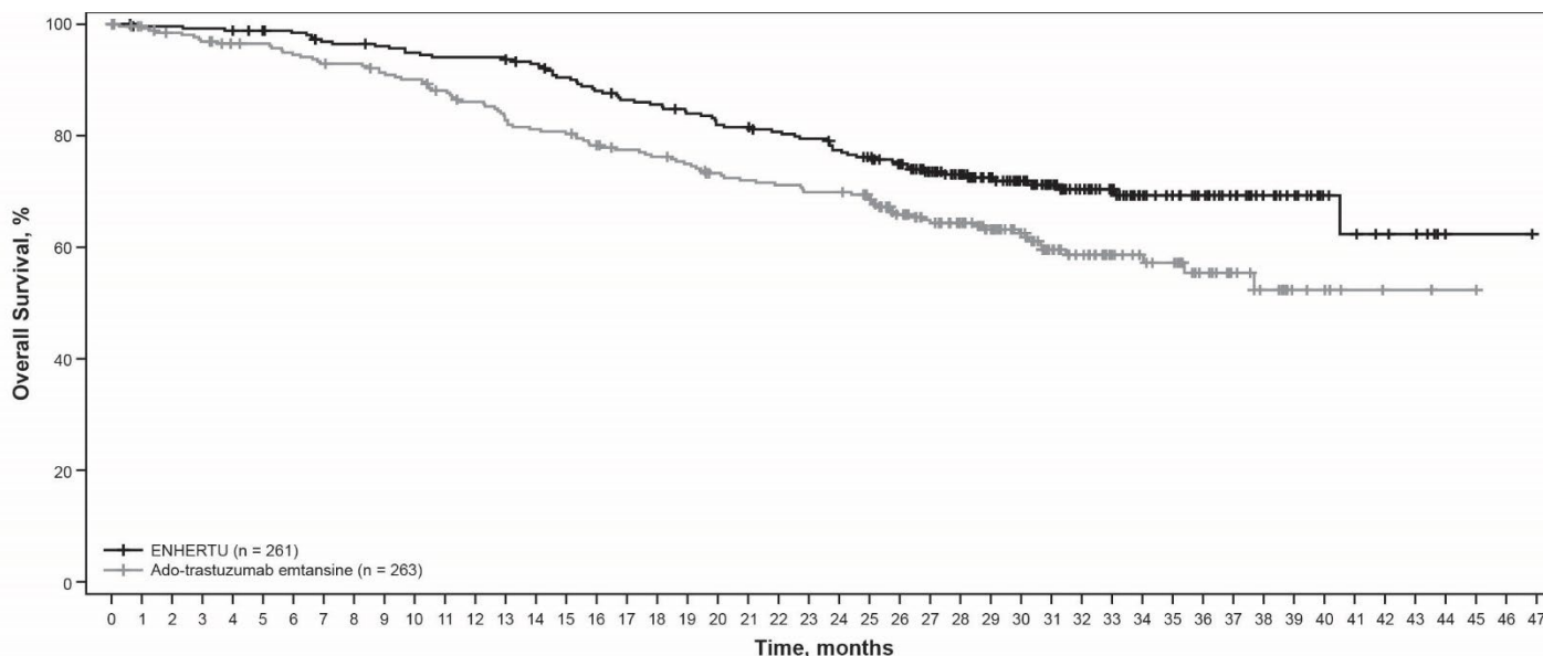
Figure 2: Kaplan-Meier Plot of Overall Survival
