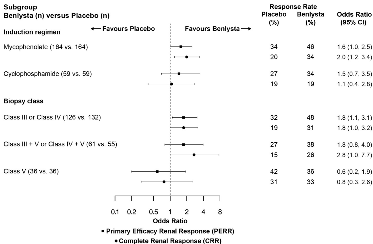
Figure 2. Odds ratio of PERR and CRR at Week 104 across subgroups
