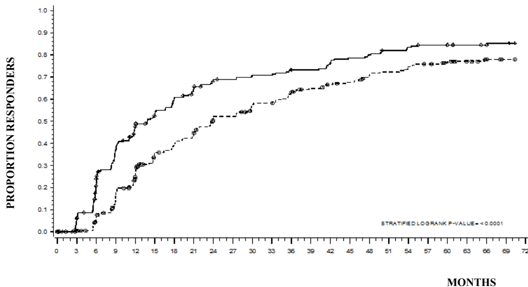
Figure 1: Kaplan-Meier estimate of time to major molecular response (MMR)
