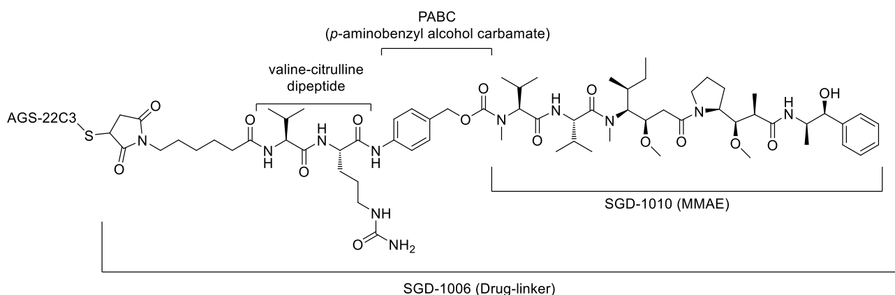
Figure 1. Structural Formula
