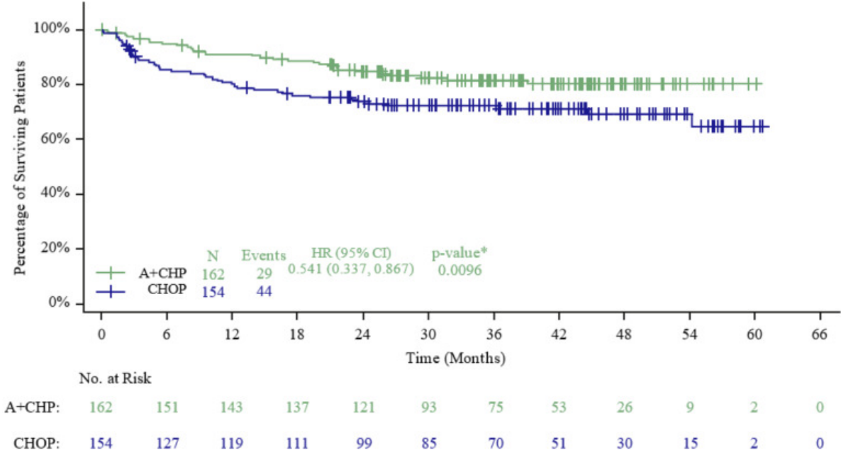
Figure 10: Overall survival in the sALCL population (ADCETRIS + CHP vs. CHOP) (primary analysis)
