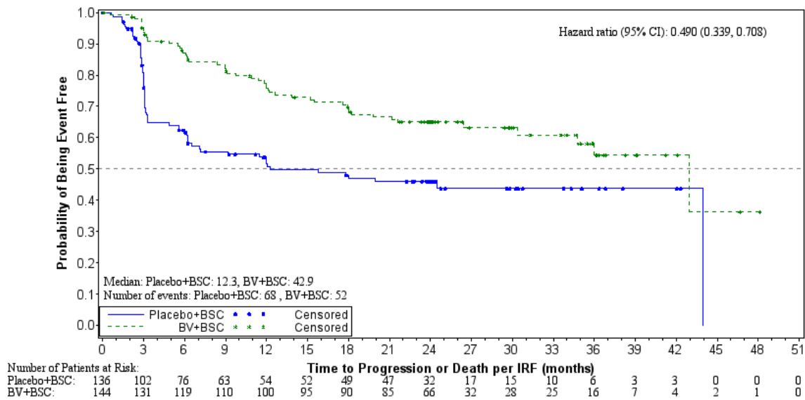
Figure 5: Kaplan-Meier Plot of PFS per IRF in Patients with \geq 2 Risk Factors (3-year follow-up)
