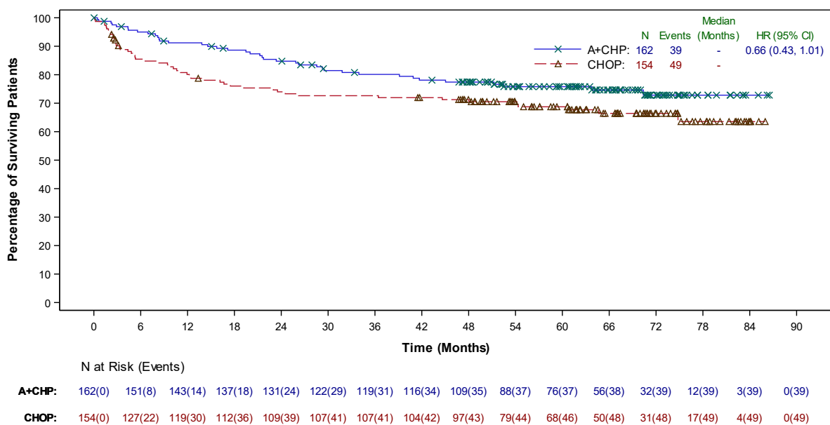
Figure 11: Overall survival in the sALCL population (ADCETRIS + CHP vs. CHOP) (study closure)
