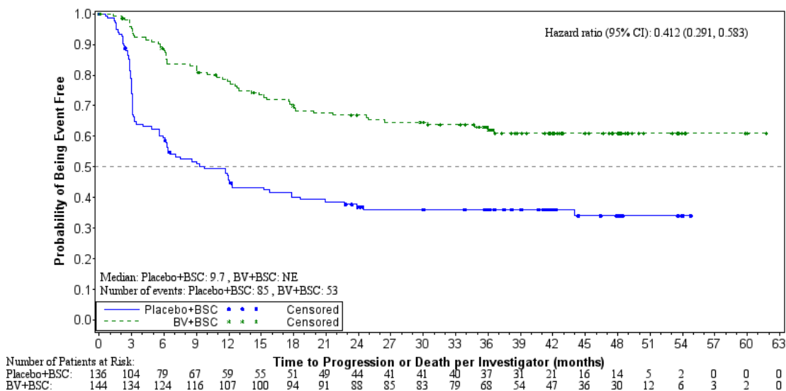
Figure 6: Kaplan-Meier Plot of PFS per Investigator in Patients with \geq 2 Risk Factors (3-year follow-up)
