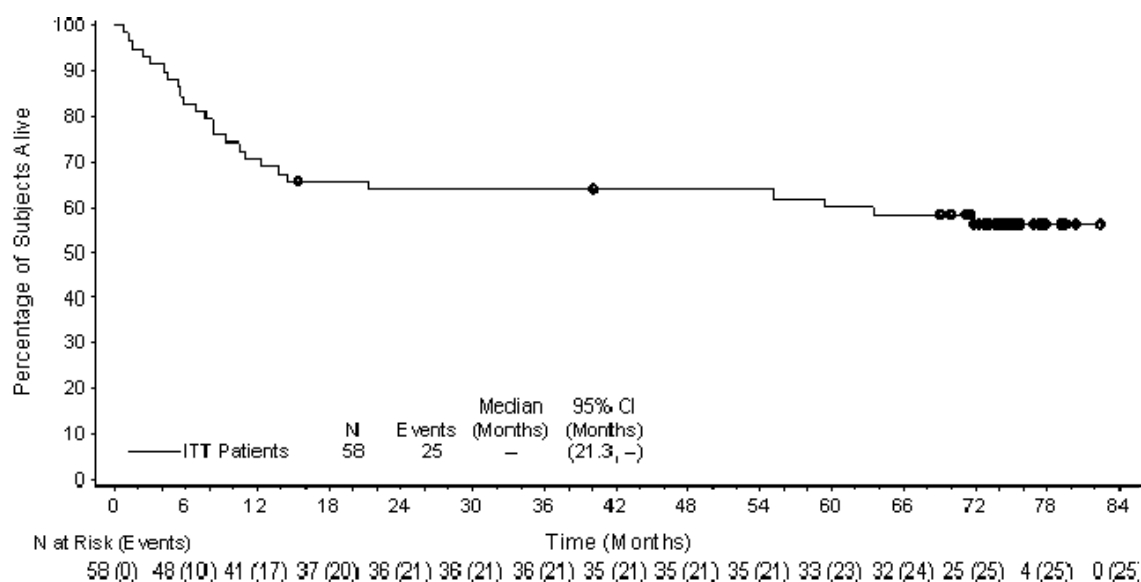
Figure 12: Kaplan-Meier Plot of OS
