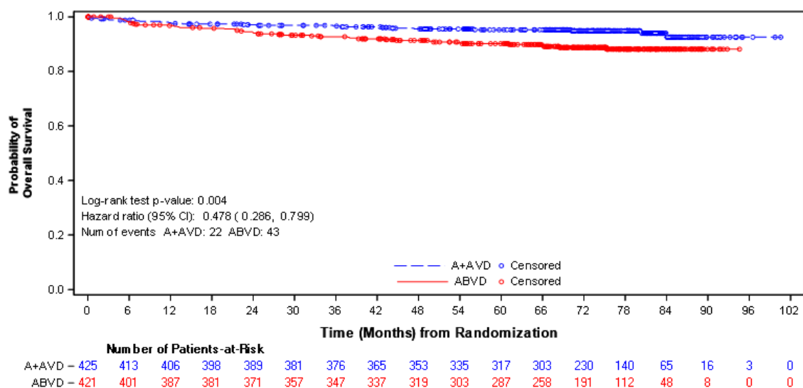
Figure 3: Overall survival in patients with Stage IV disease (ADCETRIS + AVD vs. ABVD) (6 years median follow up)
