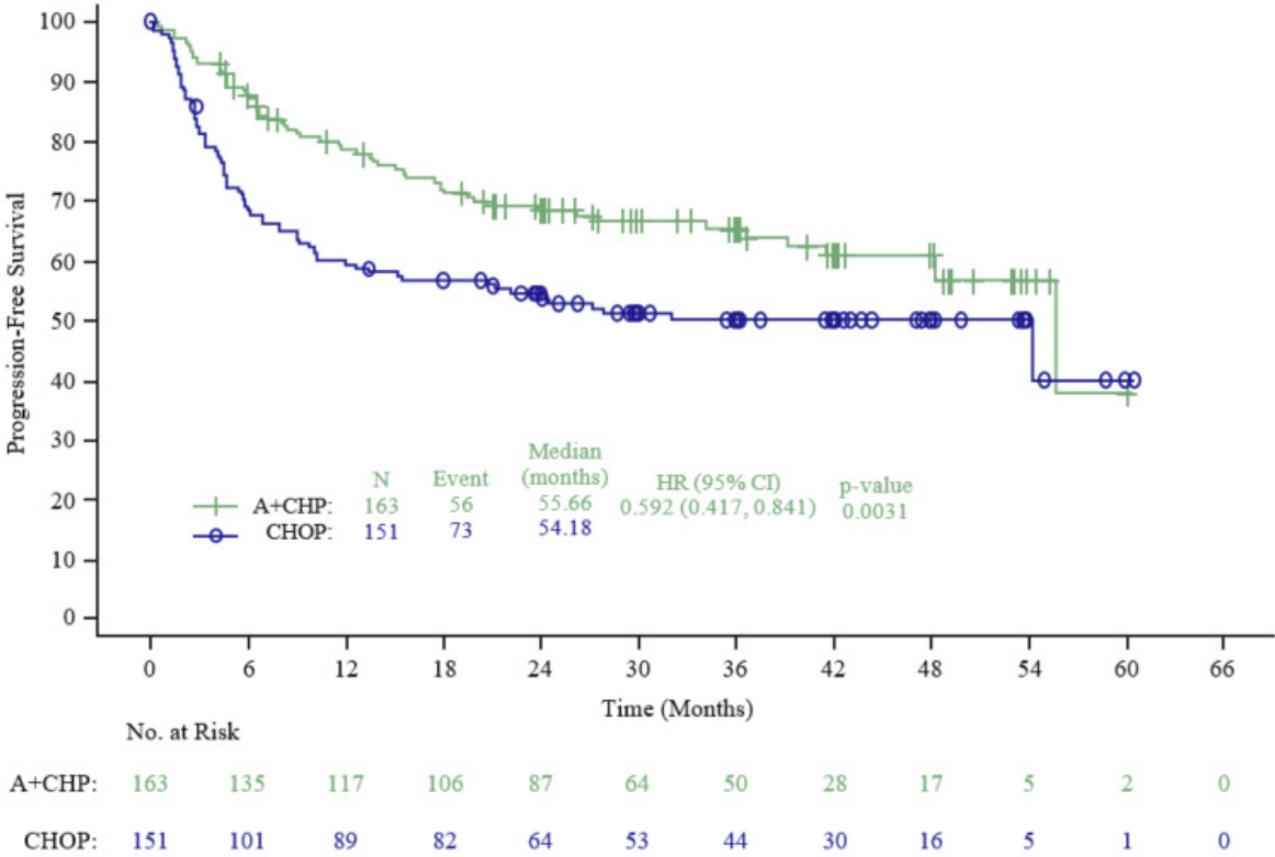
Figure 9: Progression-free survival per IRF in the sALCL population (ADCETRIS + CHP vs. CHOP) (primary analysis)
